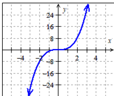
Figure 1: y = x^3
