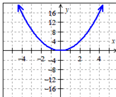
Figure 2: y = x^2
