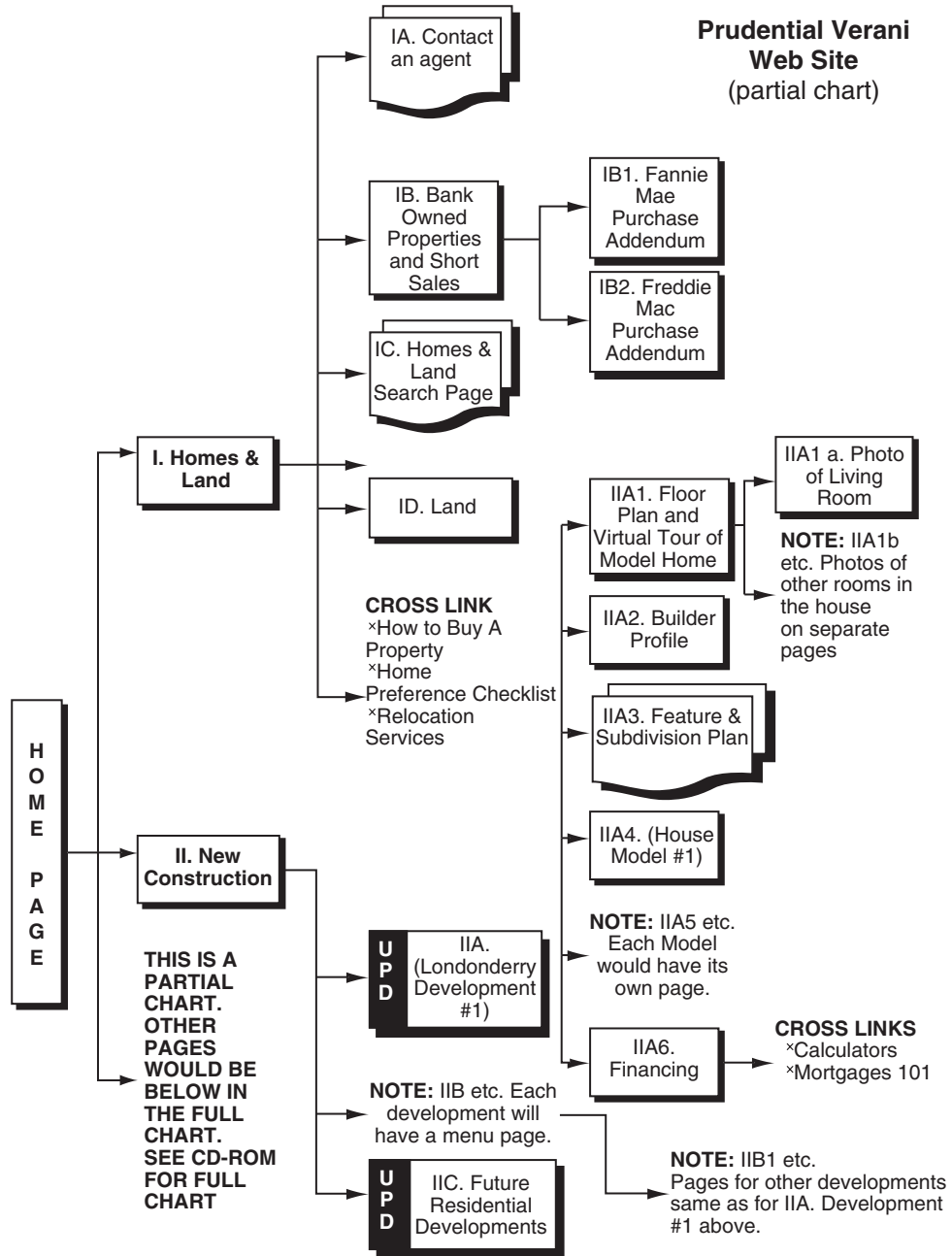
Figure 10-3 Partial flowchart/sitemap for the Prudential Verani web site.
