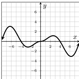
Figure 1.18: y = f(x)
