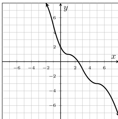
Figure 1.19: y = g(x)
