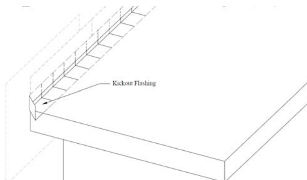
FIGURE R703.8(1) KICK-OUT FLASHING
