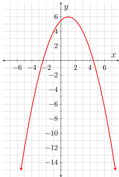
Figure 4.2.2: y = g(x)
