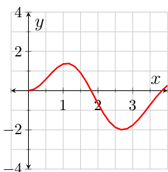
Figure 4.4.2:
