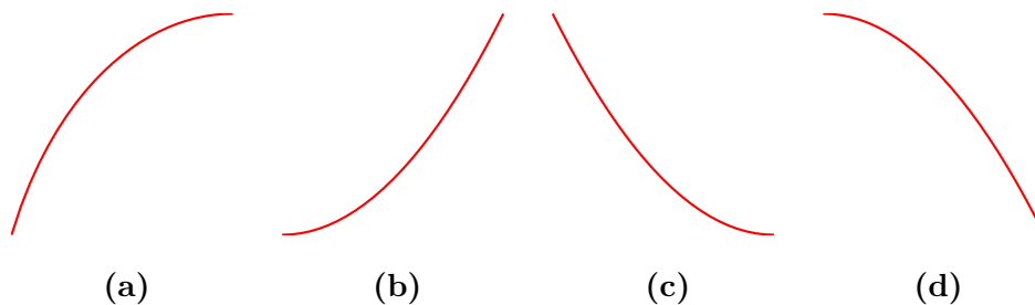
Figure 4.6.7:
