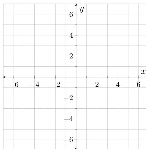
Figure 4.7.7: y = f(x)
