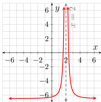
Figure 2.7.1: y = k(x) Figure 2.7.2: y = w(t) Figure 2.7.3: y = T(x)
