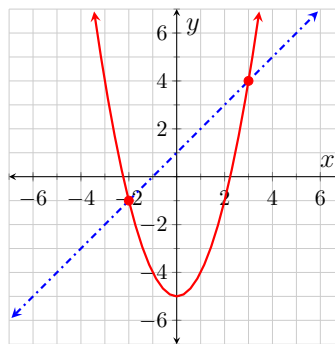
Figure 1.2.3: y = g(x) = x^2 - 5 and a secant line
