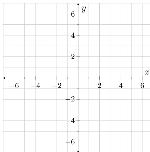
Figure 4.6.2: y = f(x)
