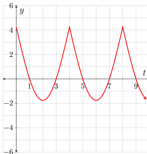
Figure 4.7.2:
