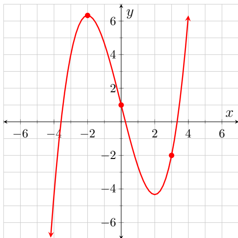
Figure 4.2.4: y = f(x)
