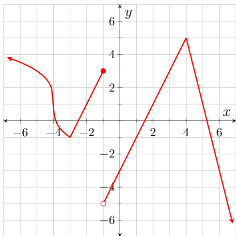
Figure 4.3.1: y = k(x)
