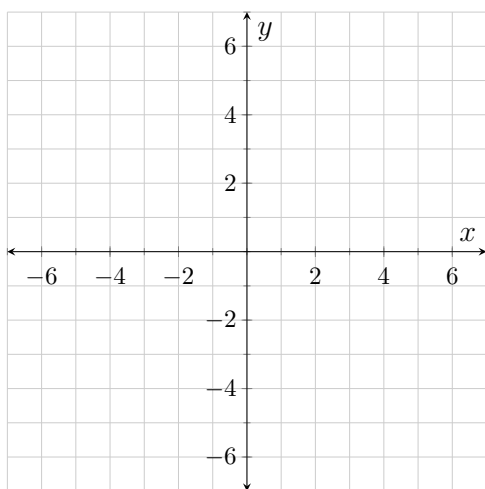
Figure 4.5.7:
