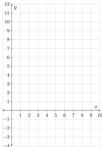
Figure 4.2.15: y = w'(x)
