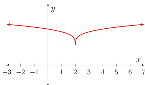
Figure 9.1.2: mystery curve 2
