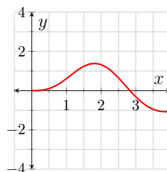
Figure 4.4.5:
