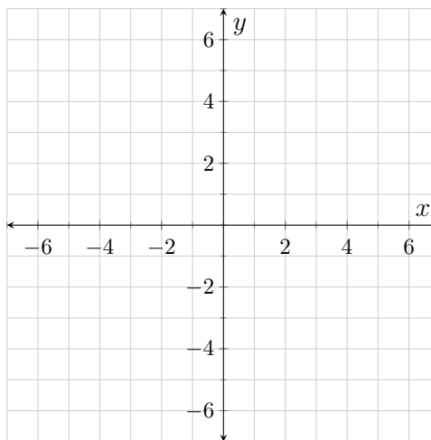
Figure 4.3.2: y = k'(x)
