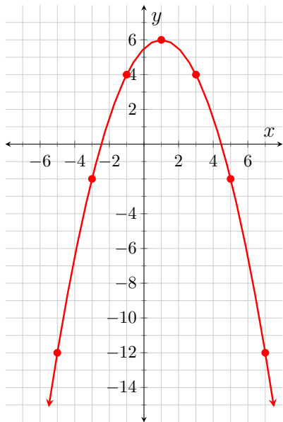
Figure 4.2.1: y = g(x)
