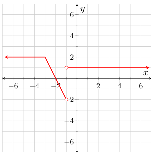
Figure 4.5.5: y = f(x)
