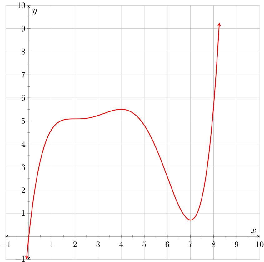
Figure 4.2.12: y = w(x)
