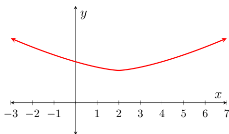
Figure 9.1.1: mystery curve 1
