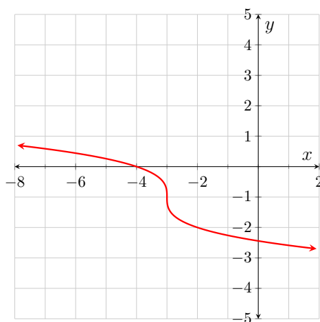
Figure 9.2.2: y = g(x)
