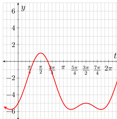
Figure 5.12.2: y = g(t)
