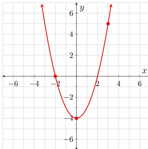
Figure 4.2.5: y = f'(x)
