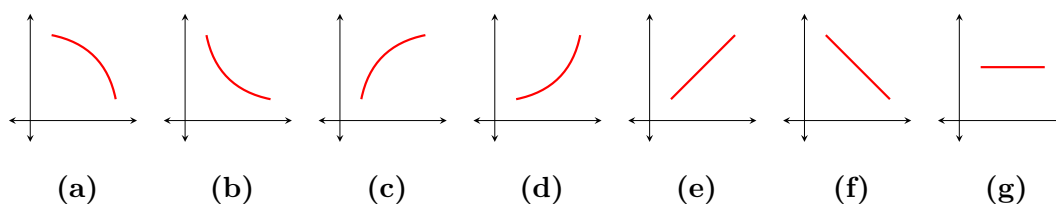
Figure 4.7.1: Seven curves
