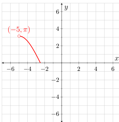
Figure 4.3.4: y = g'(x)
