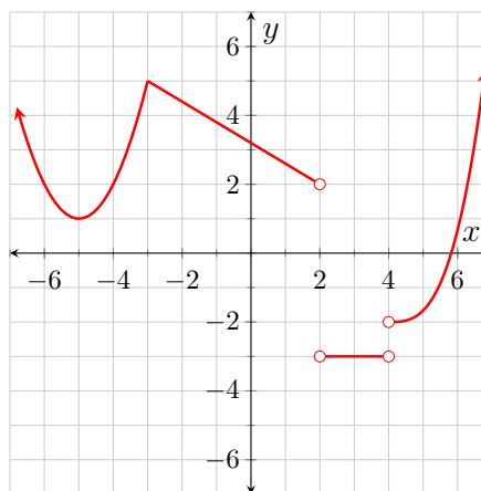
Figure 4.5.11: y = g'(x)
