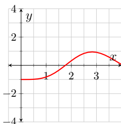
Figure 4.4.3:
