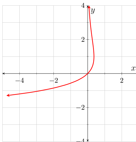
Figure 7.1.3: y = xe^y
