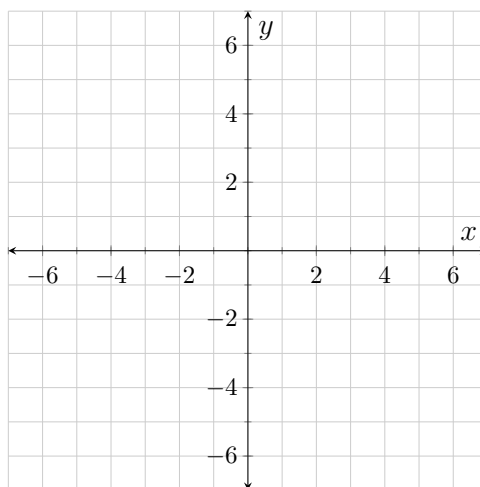
Figure 4.2.11: y = g'(x)
